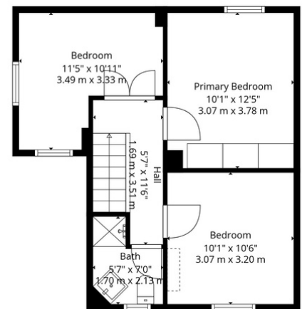
Floor 3
